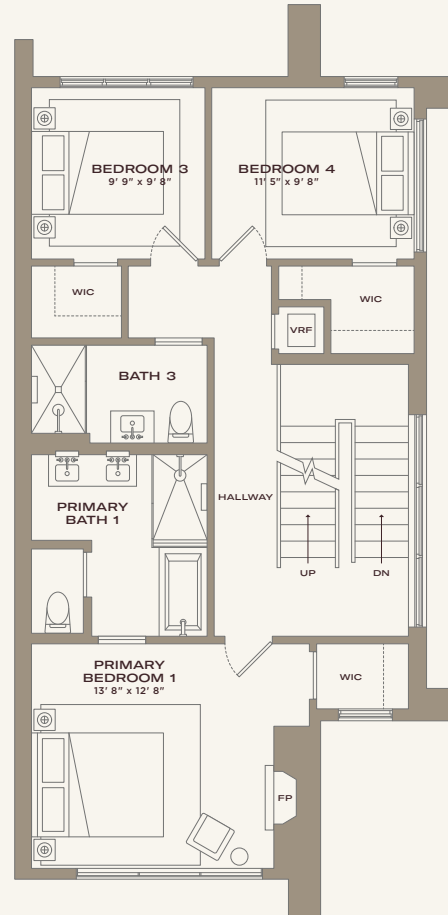
THIRD FLOOR
